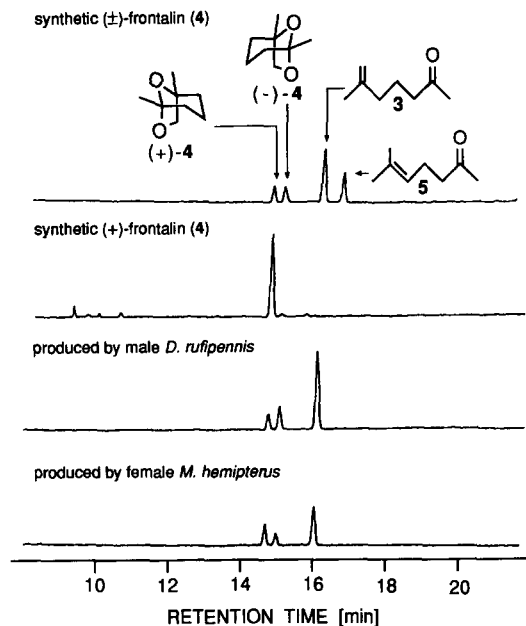
Figure 4. GC analyses of synthetic (±)- and (+)-frontalin (4), and 4 produced by D. rufipennis and M. hemipterus during vapor exposure to 6-methyl-6-hepten-2-one (3). Traces for male and female beetles were virtually identical. Exposure of female D. ponderosae to deuterio-3 resulted in the production of racemic deuterio-4. Chromatography: Cyclodex-B column; 80 °C isothermal; split injection; linear flow velocity of carrier gas: 35 cm/s; injector temperature: 200 °C.
